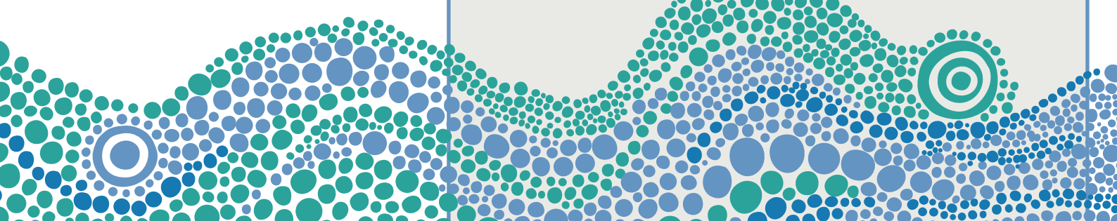
Figure 1. ACCHOs located in hot zone areas
